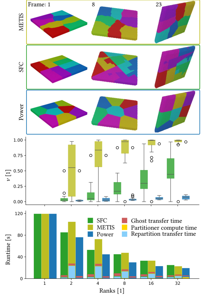
Fig. 8. Turntable . A rectangular domain is rotated rapidly for 24 frames, where we perform a Poisson solve followed by an Eulerian advection step. Partitionings for frames 1, 8, and 23 are shown (top); METIS produces similar partitionings every frame, but they shift in time; SFC creates non-local partitionings when the domain is non-axis aligned (see frames 8 and 23); Power (ours) produces local and temporally stable partitionings. The temporal index v is recorded for every frame in a box plot (middle), together with the total runtime (bottom). © Wētā FX Ltd.
