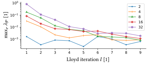
Fig. 5. Power partitioner convergence plot. We study the convergence of the Lloyd iteration loop in Alg. 1. The domain subset is a box with \lfloor \sqrt[3]{10^4 R} \rfloor buckets on all sides to keep the size of each partition P_r roughly equal. We set \tau_{\text{load}} = 0 to ensure the break in Alg. 1 is never triggered and we vary the number of ranks R = \{2, 4, 8, 16, 32\} . © Wētā FX Ltd.
