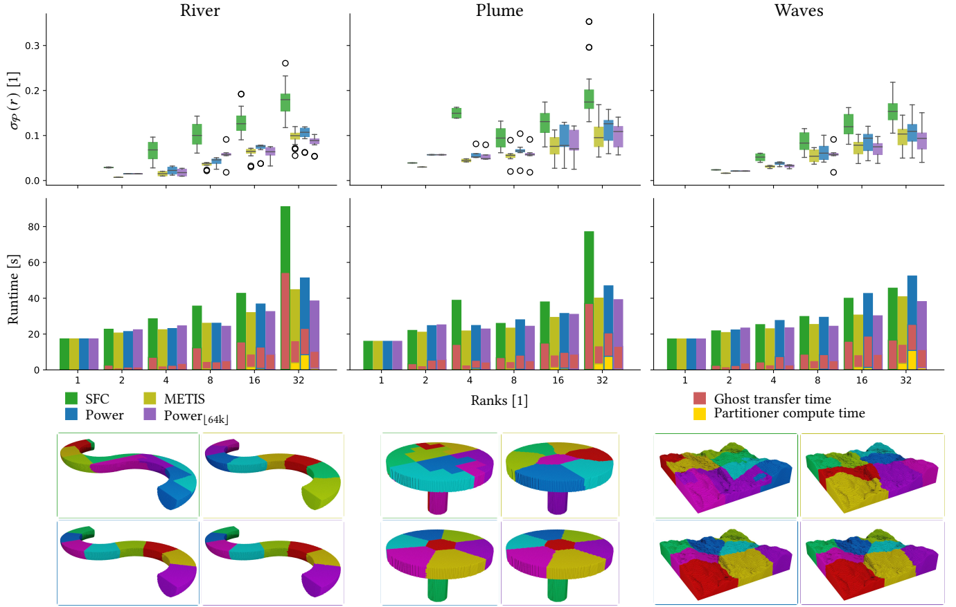
Fig. 10. Weak scaling. Results from the River, Plume, and Waves weak scaling examples are shown, comparing different partitioning algorithms on a static domain, where we perform a Poisson solve followed by an Eulerian advection step. We provide the surface index \sigma_P(r) (Eq. 19) from the final frame (top row), as well as performance numbers (middle row) from the frame with the lowest total runtime (out of 10 frames). We explicitly mark the time spent computing the partitioning and time spent transferring ghost data. Since the domain is static, we do not provide the temporal consistency index. For a visual comparison we also visualize the partitionings for 8 machines; the color of the image border indicates what algorithm was used. Performance metrics for these simulations are summarized in Tab. 4. © Wētā FX Ltd.
