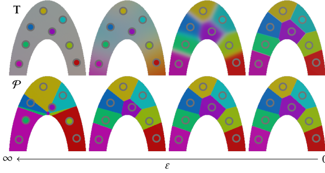
Fig. 4. Effect of regularization on Power partitioning. The coupling T (top) and resulting partitioning P (bottom) is visualized for varying \varepsilon on a non-convex domain. Ranks are drawn as circles with color \gamma_r . In the top row, the color is computed on buckets as \gamma_b = (\sum_r \gamma_r T_{rb}) / \|\sum_r \gamma_r T_{rb}\|_2 . In the bottom row the color is computed as \gamma_b = \gamma_{P(b)} . © Wētā FX Ltd.
